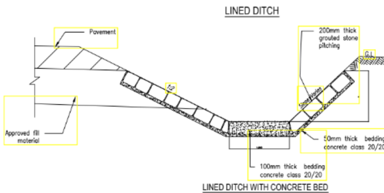
Figure 14 Lined Ditch
