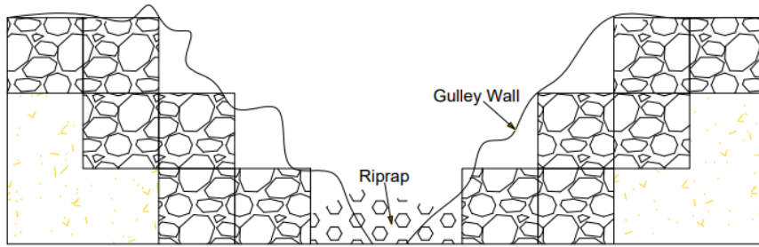
Figure 13 Gulley Protection Works
